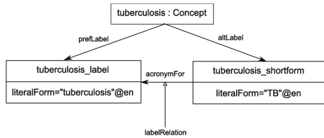
Figure 1.1: Taken from McCrae, John, et al. (2012). Interchanging lexical resources on the Semantic Web. Language Resources and Evaluation. 46. 701-719. 10.1007/s10579-012-9182-3.
