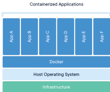
Figure: www.docker.com/resources/what-container/
