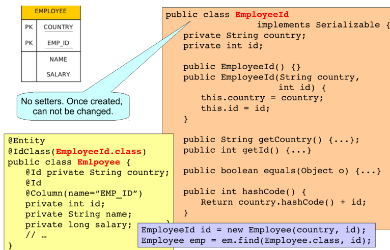
Figure 16: Id Class
