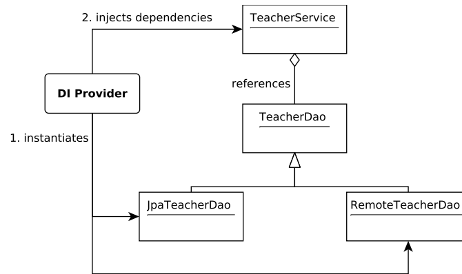
Figure 7: Dependency injection principle.
