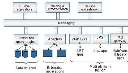
Figure 3: ESB architecture. Source: https://docs.oracle.com/cd/E23943_01/doc.1111/e15020/img/esb_architecture.gif
