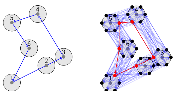
Trying each of the k possible starting locations
