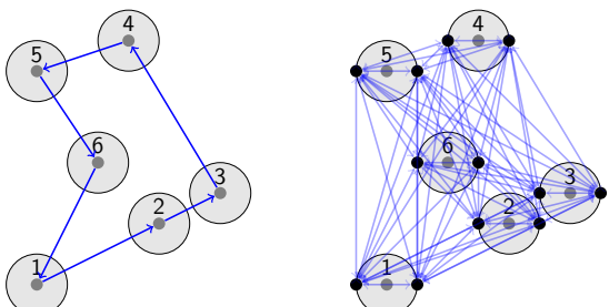
The discretized variant of the TSPN can be formulated as the GTSP
