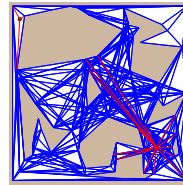
Visibility graph
