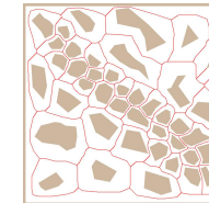
Voronoi diagram
