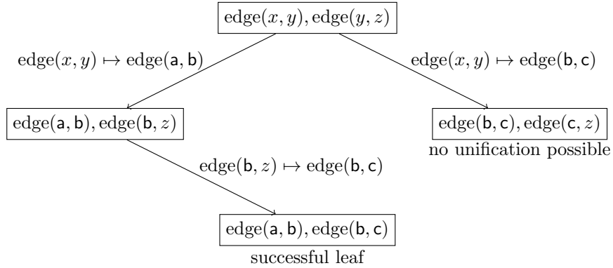
Figure 12: By searching this tree, the substitution \{x \mapsto a, y \mapsto b, z \mapsto c\} is found unifying all the negative literals of (104) with elements of (106).
