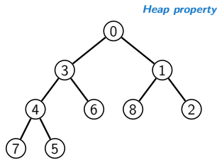
Heap property
