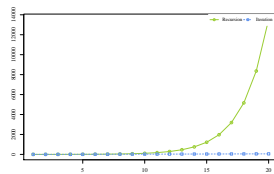
fibonacci-n20.pdf
