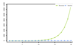
fibonacci-n20.pdf
