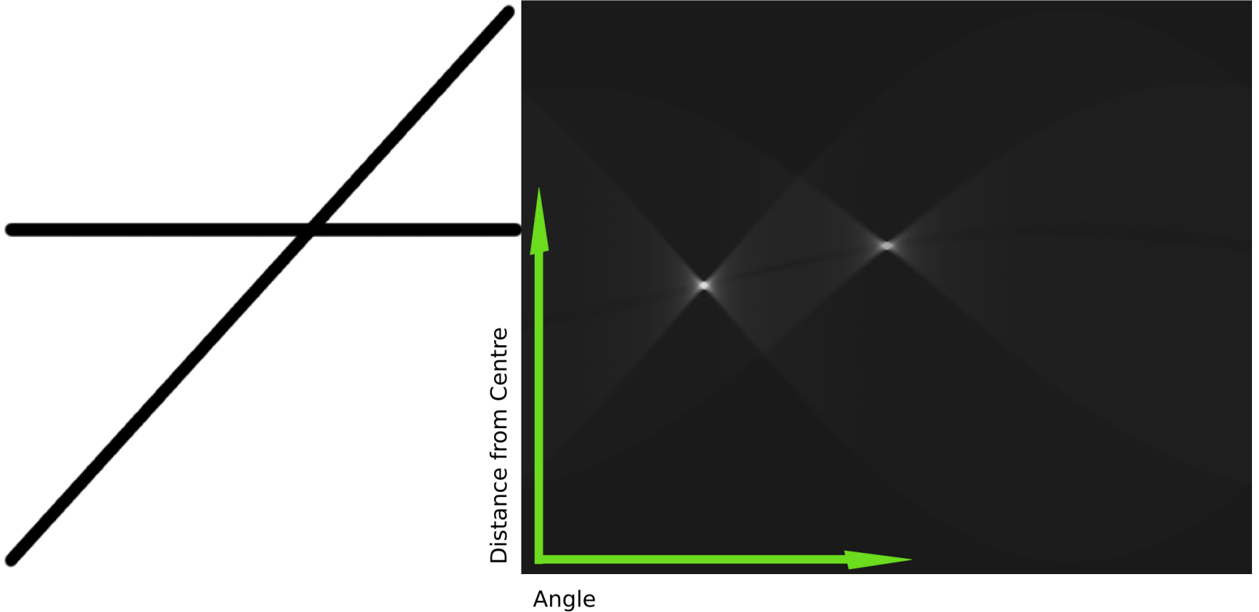
Input Image
