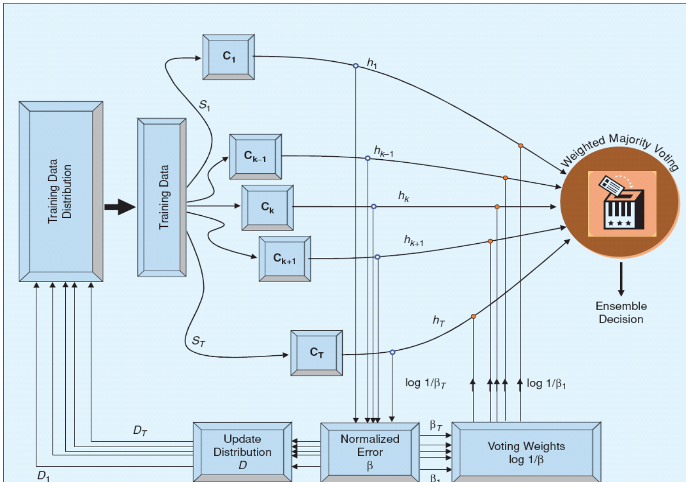
Figure 9. The AdaBoost.M1 algorithm.
