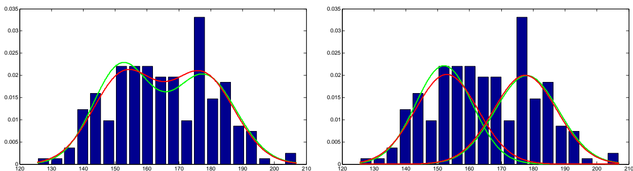
Figure 2: Expected results from task 2. Theoretical probability density is shown in red colour, estimated probability density is shown in green colour.
