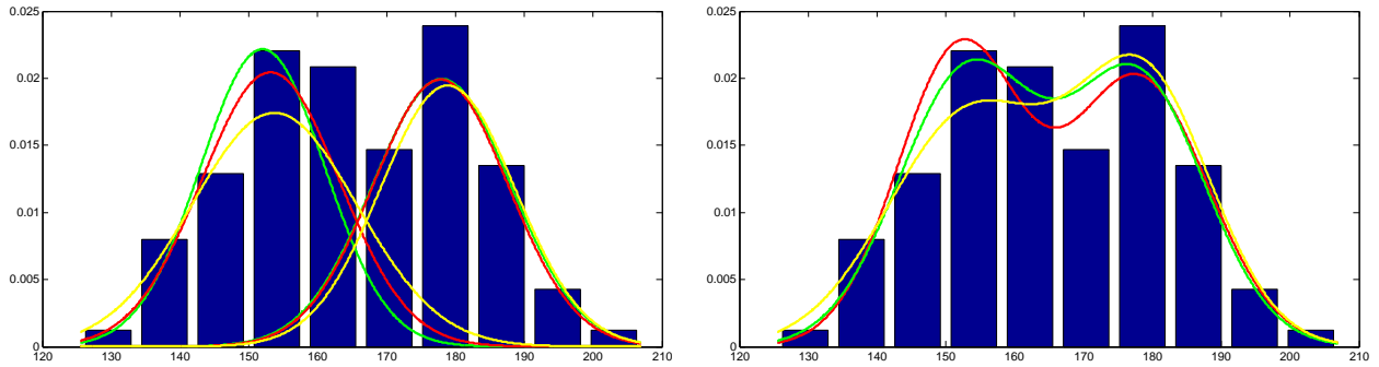
Figure 3: Expected result from task 3. Theoretical probability density is shown in red colour, probability density estimated using EM algorithm is shown in green colour, probability density estimated only from annotated samples is shown in yellow colour.
