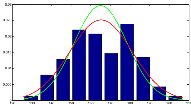
Figure 1: Expected result from task 1. Theoretical probability density is shown in red colour, estimated probability density is shown in green colour.
