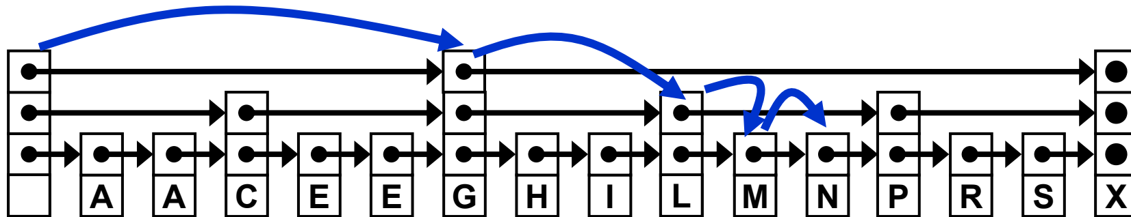
A linked list with even faster search capability
