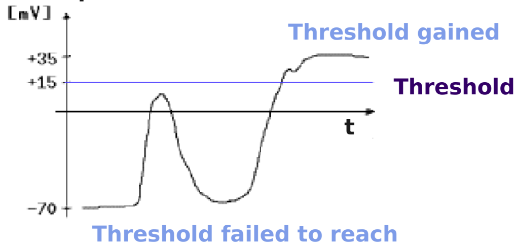
Neuron's potential
