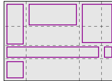
GridBagLayout
