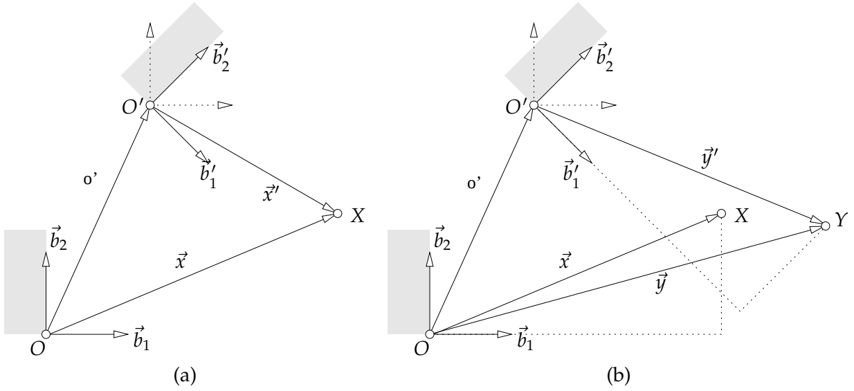
Figure 5.1: Representation of motion. (a) Alias representation: Point X is represented in two coordinate systems. (b) Alibi representation: Point X move together with the coordinate system into point Y .
