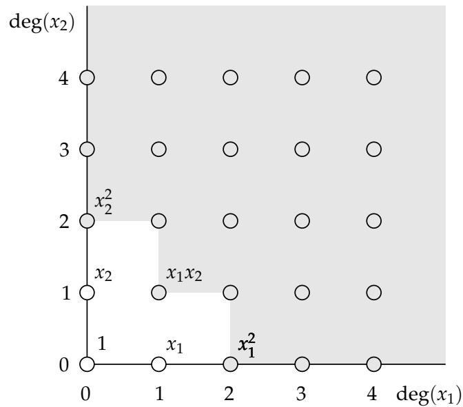
Figure 3.6: Standard monomials x_1, x_2, 1 of G from Equation 3.25 are not divisible by leading monomials x_1^2, x_1x_2, x_2^2 of G . All other monomials, shown in gray, are divisible by at least one of the leading monomials of G .
