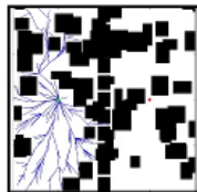
Informed RRT*
