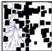
Informed RRT*
