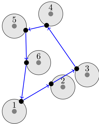
A solution of the CETSP
