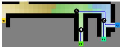
Greedy assignment of goal candidates (frontiers)
