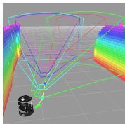
Detect and cluster frontiers
