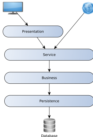
Figure: Layered system architecture.
