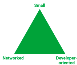
Figure 3: https://www.nginx.com/blog/principles-of-modern-application-development
