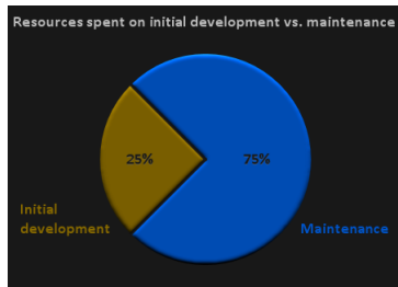
Figure 1: http://clarityincode.com/software-maintenance
