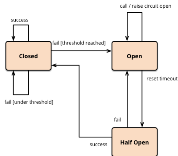
Figure 12: Circuit Breaker states.
