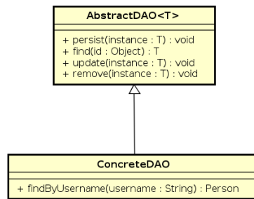
Figure 9: Common Data access object hierarchy.
