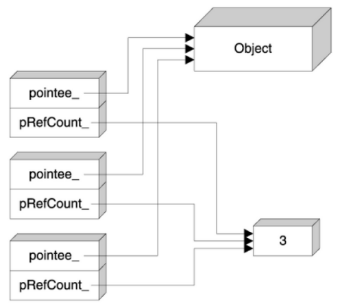
image source: https://stackoverflow.com/questions/9200664/how-is-the-stdtr1shared-ptr-implemented
