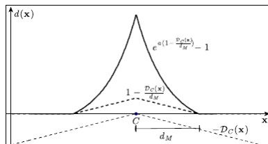
Fig. 3. The function d in the case of \mathbf{x} \in \mathbb{R} . If a centerline point is located in C , the function we want to learn is obtained from the distance transform D_C , after thresholding and scaling. The vertical axis has been scaled for visualization purposes.
