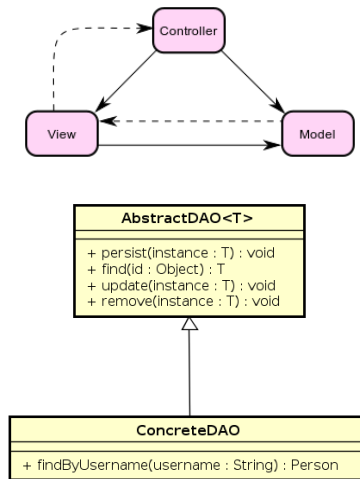
Figure 9: Common Data access object hierarchy.
