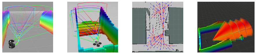
Detect and cluster frontiers Sampled poses to cover a cluster Paths to the sampled poses
