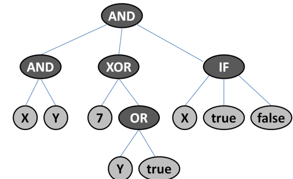
Logic expression
