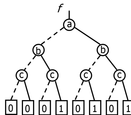
Decision tree
