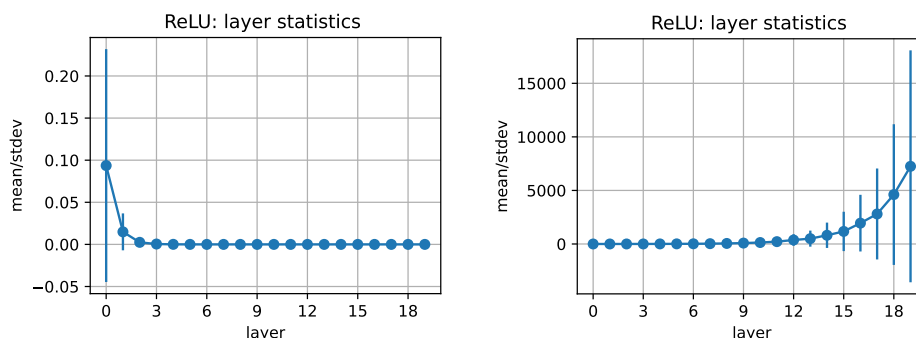
Figure 1: Unit statistics in a 20-layer ReLU neural network with weights initialized with standard deviation 0.01 ( left ) and 0.1 ( right ).
