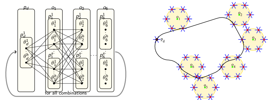
Dubins Touring Region Problem (DTRP)
