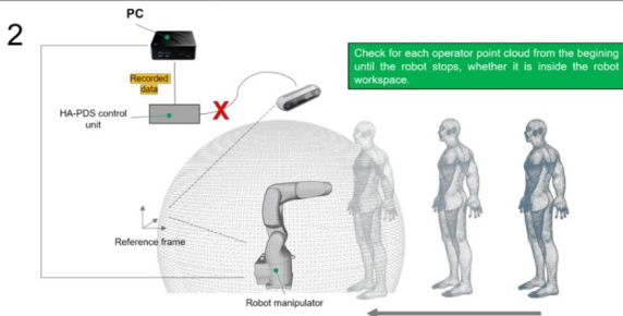
Figure 2: Method to test the HA-PDS for maintaining a safe distance to humans.
