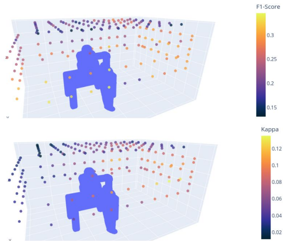
Fig. 7: RGB-D camera placement heatmap for 'robot' space in Scene 3; F_1 (top) and \kappa (bottom) values.
