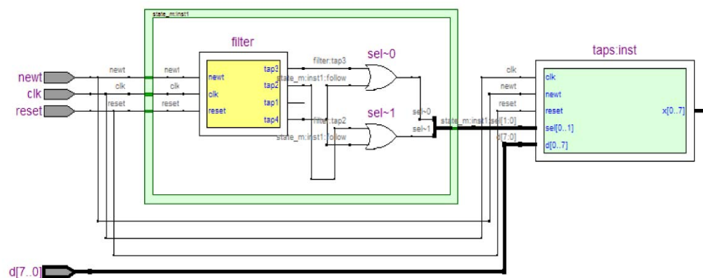
Figure 12-24. Filtering Across Hierarchical Boundaries, Large Example
