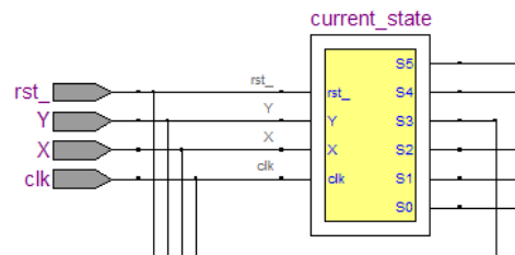
Figure 12-32. State Machine Instance in RTL Viewer Schematic View
