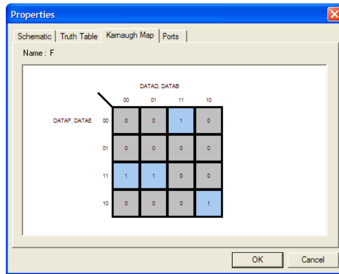
Figure 12-11. Karnaugh Map Tab
