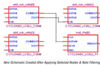
Figure 12-22. Selected Nodes and Nets Filtering on Figure 12-21 Schematic
