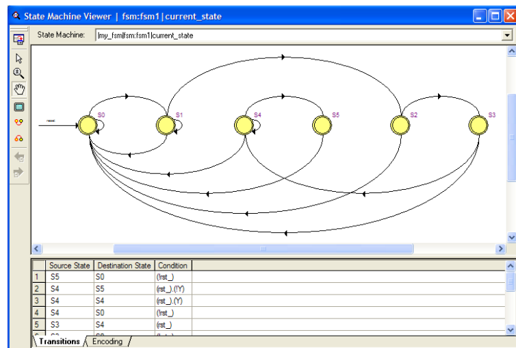
Figure 12-35. State Machine Viewer Showing Correct Transitions
