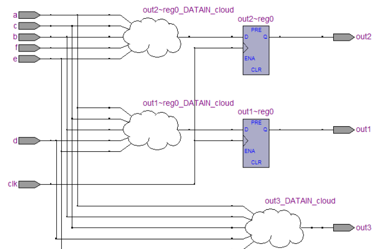
Figure 12-13. Schematic After Combinational Logic Grouping
