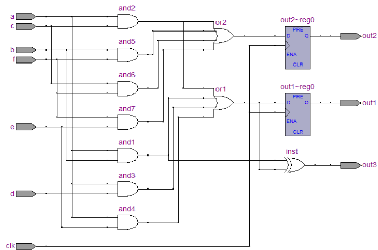
Figure 12-12. Schematic Before Combinational Logic Grouping
