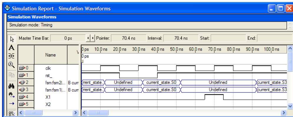
Figure 12-31. Simulation Result Showing Undefined States
