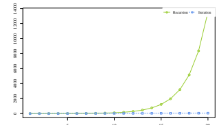
fibonacci-n20.pdf
