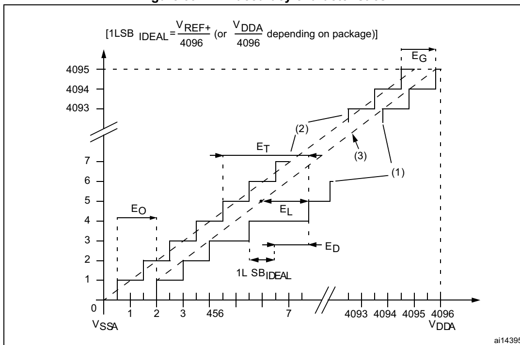
Figure 39. ADC accuracy characteristics
