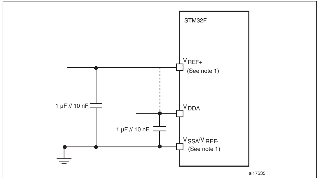
Figure 41. Power supply and reference decoupling ( V_{REF+} not connected to V_{DDA} )
