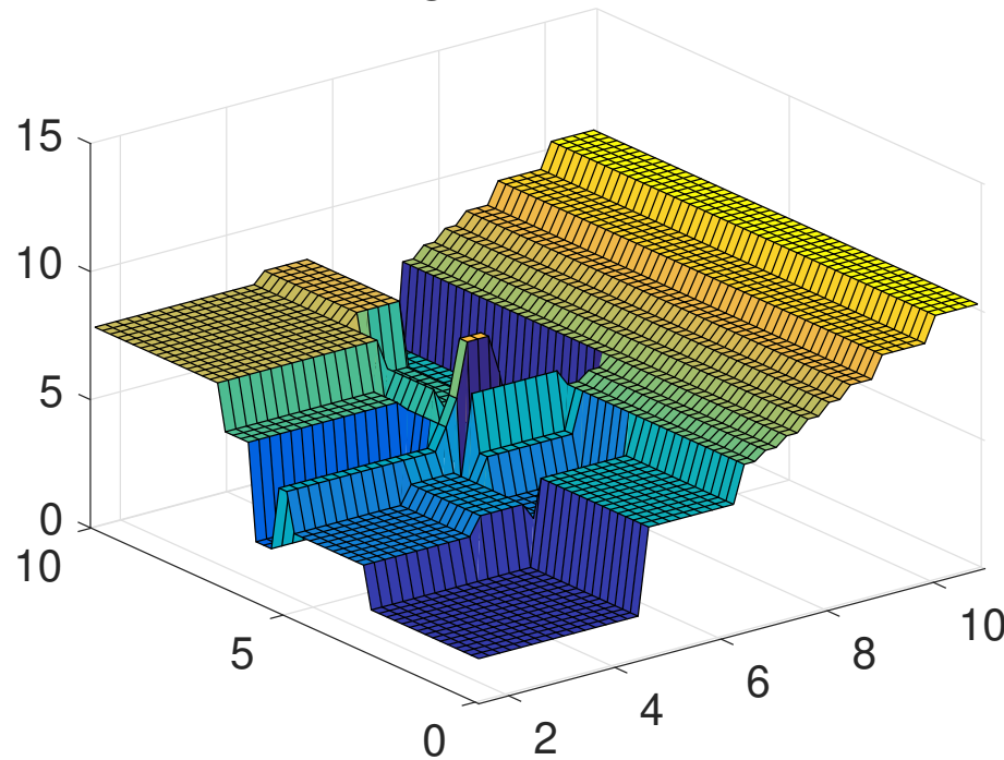
Regression tree
