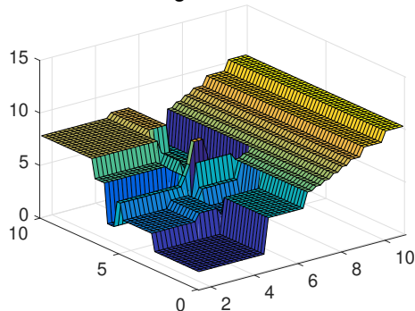
Regression tree
