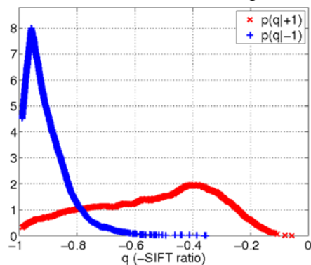
SIFT-ratio (only)
