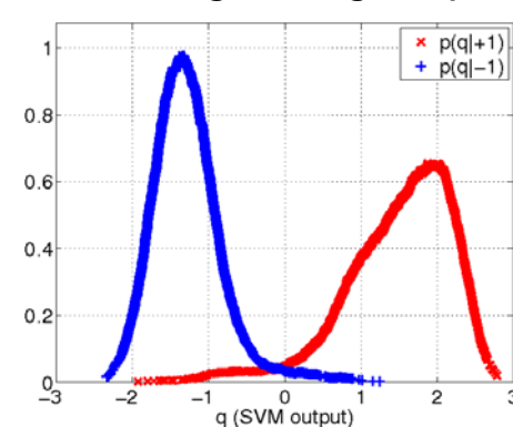
1000 growing steps
