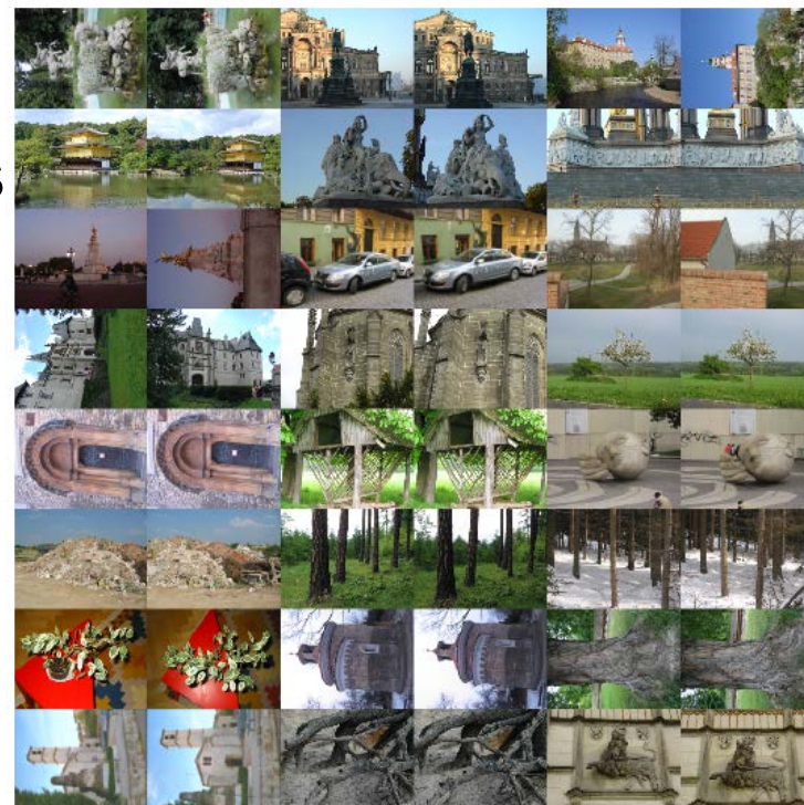
100 growing steps
