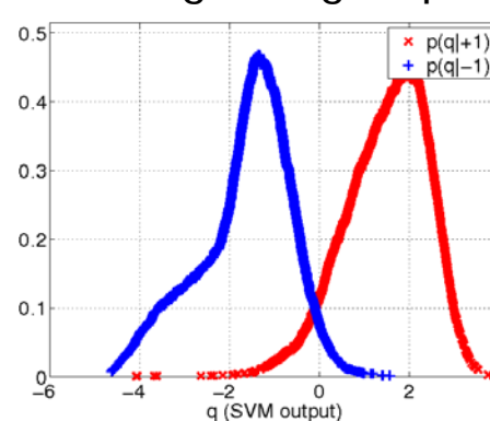
100 growing steps
