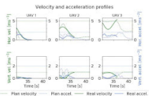
Orienteeing Problem with Bézier curves: Non-crossing field experiment with 3 multi-rotor drones
