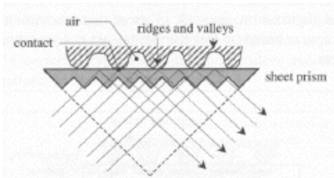
Internal reflection optical sensor
