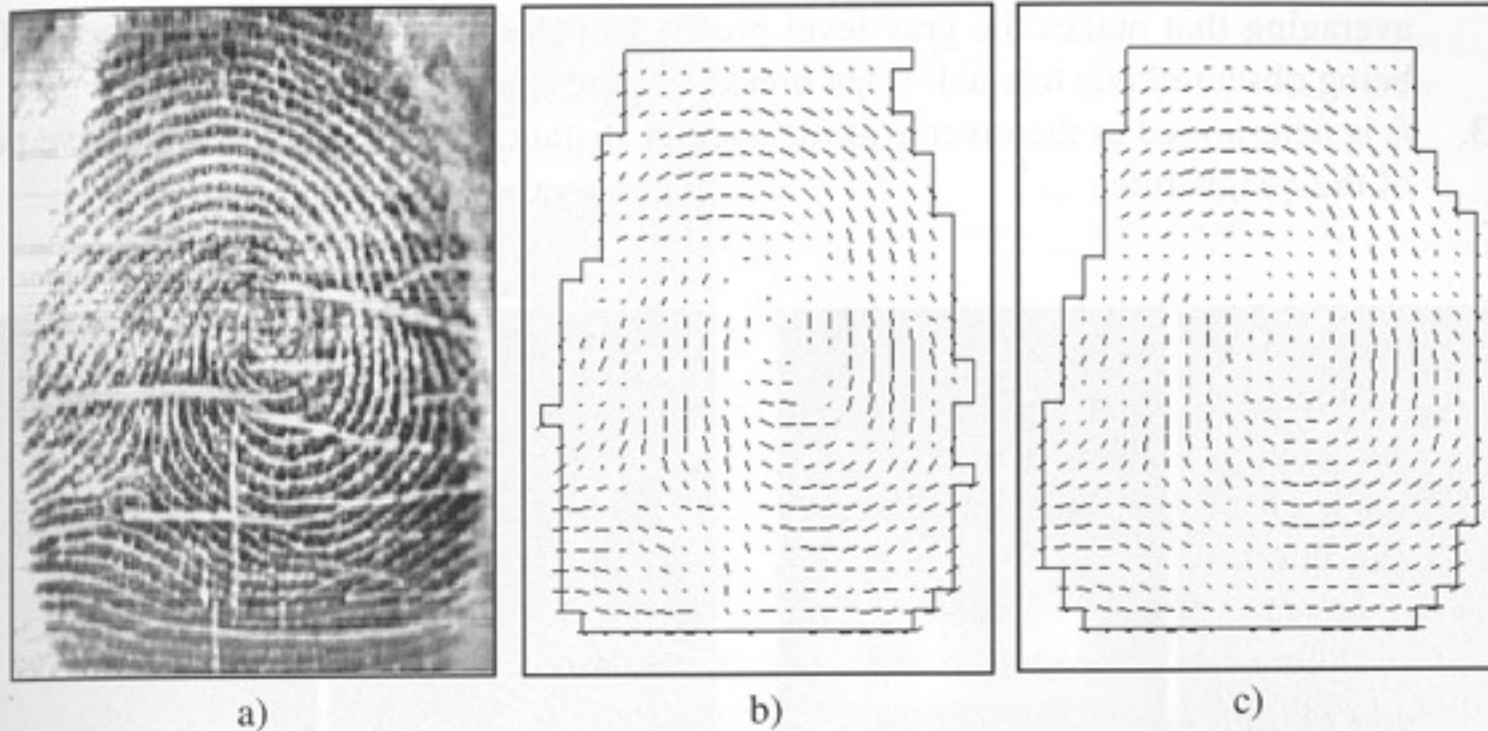
Figure 3.9. a) A poor quality fingerprint image; b) the orientation image of the fingerprint in a) is computed through the Donahue and Rokhlin (1993) method; the orientation of several elements is clearly inconsistent and a regularization step appears necessary; c) the orientation image is the result of the local averaging of each element in b) in its 3 \times 3 window according to Equation (2).
