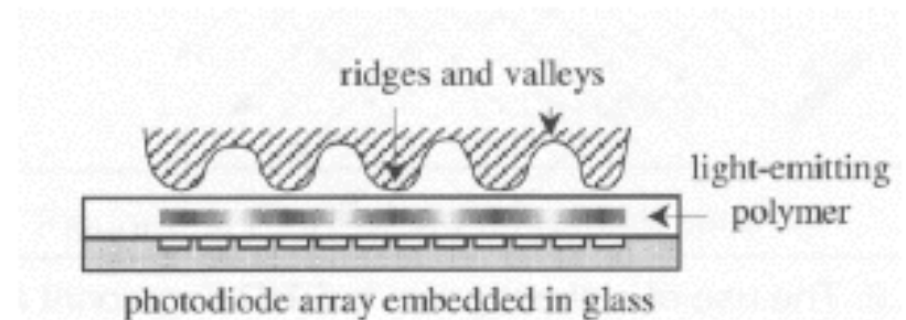
Electro-optical fingerprint sensor
