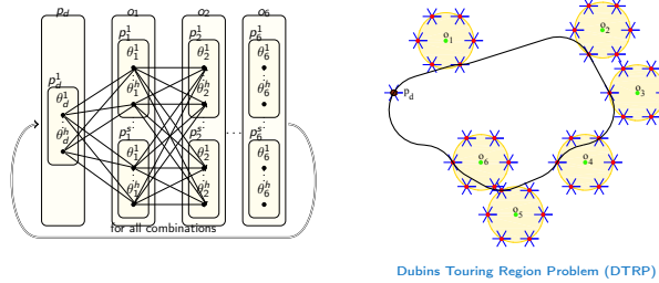
Dubins Touring Region Problem (DTRP)
