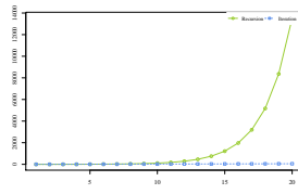
fibonacci-n20.pdf
