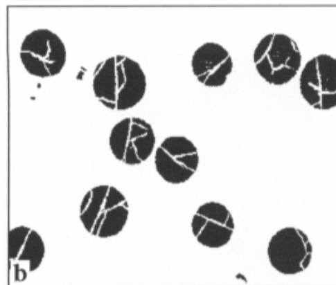
Thresholded
