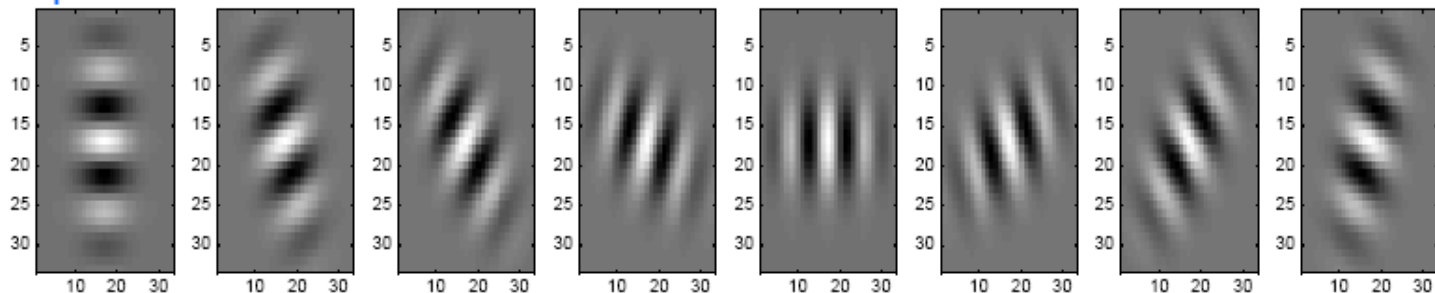
Fingerprint 1
