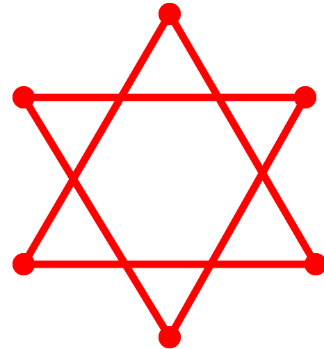
Disconnected graph
