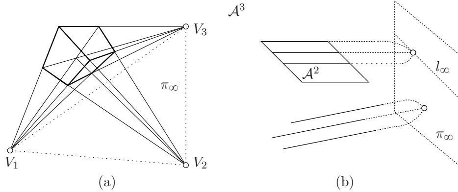
Figure 10.1: (a) A perspective image of a cube generates three vanishing points V_1 , V_2 and V_3 and hence also three vanishing lines l_{12} , l_{23} and l_{31} . (b) Every plane adds one line of ideal points to the three-dimensional affine space. Every ideal point corresponds to one direction, i.e. to a set of parallel lines. Each ideal line corresponds to a set of parallel planes.
