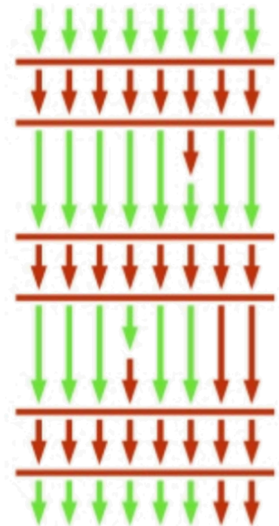
Garbage-First
